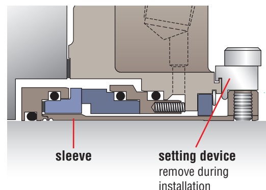
Cartridge pusher seal
