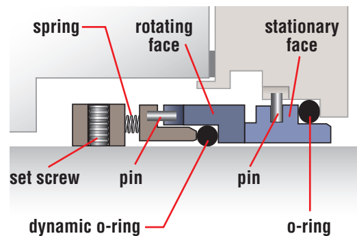
Component pusher seal
