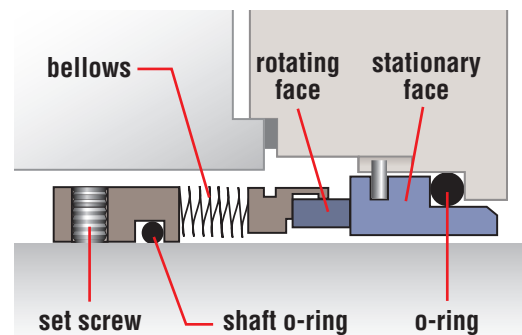
Component metal bellows seal
