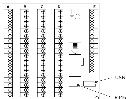
Module positions
